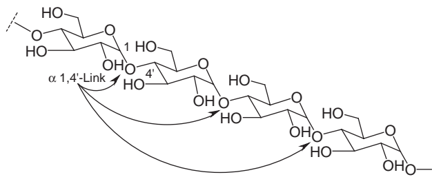
A partial structure of amylose
