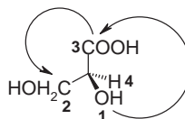
( S )-2,3-Dihydroxypropanoic acid Priority order 1 to 4 is in clockwise direction
