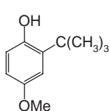
Butylated hydroxyanisole (BHA)
