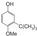
Butylated hydroxyanisole (BHA)
