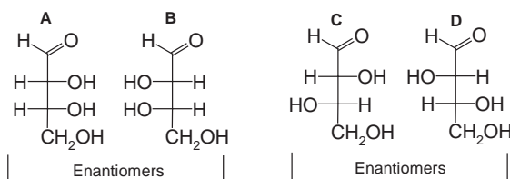
Four possible stereoisomers of 2,3,4-trihydroxybutanal
