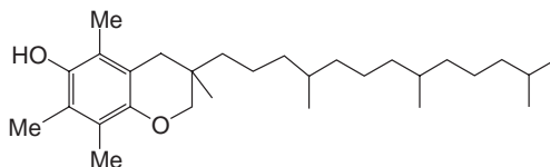
Vitamin E \alpha -Tocopherol
