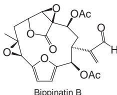
Bippinatin B
