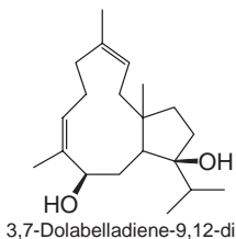
3,7-Dolabelladiene-9,12-diol
