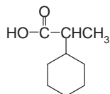
2-Cyclohexylpropanoic acid
