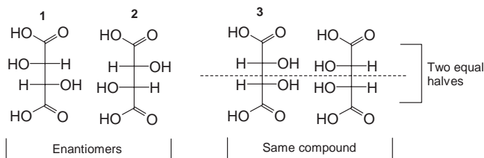
Stereoisomers of tartaric acid
